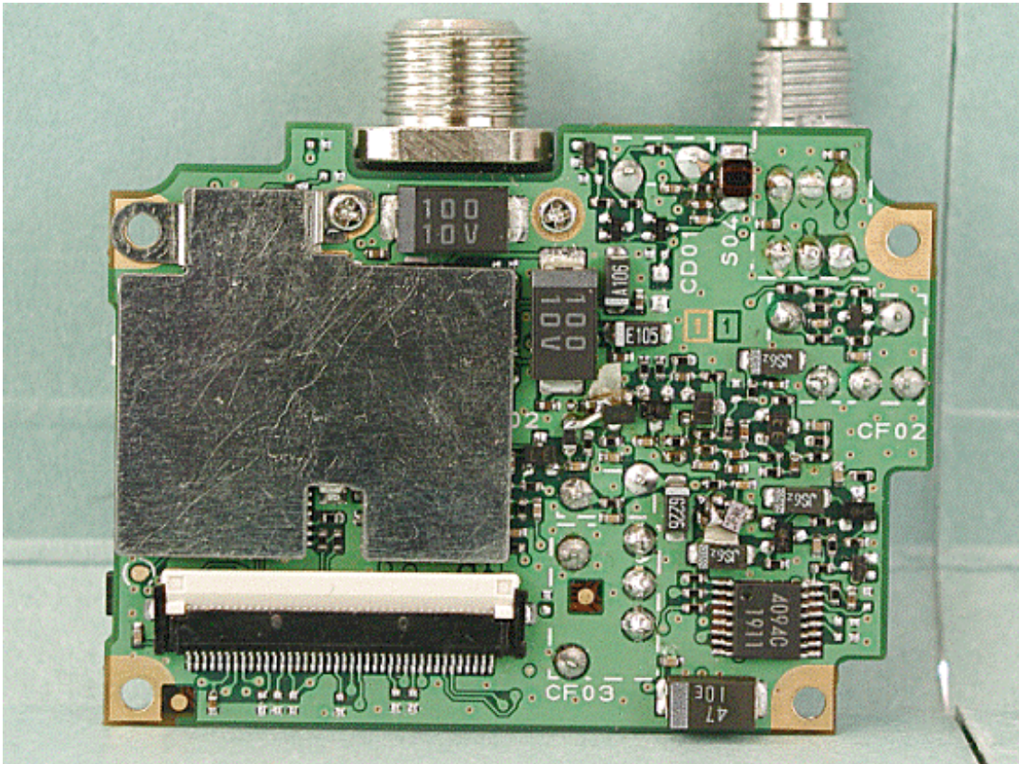
Side-B of AF-UNIT with Shield Plate
