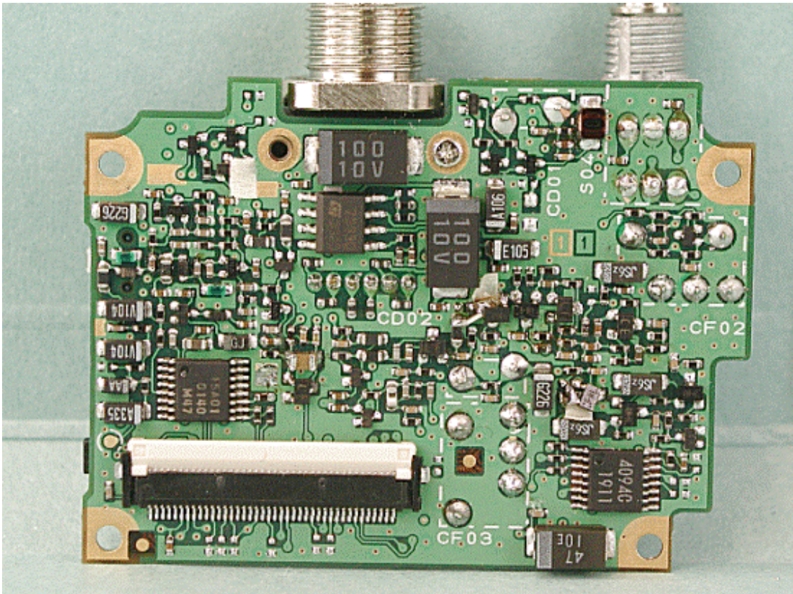
Side-B of AF-UNIT without Shield Plate
